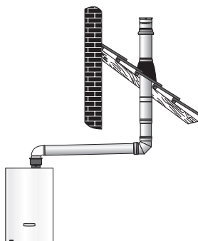
C33 - VERTICALE (Ø 80/125)
